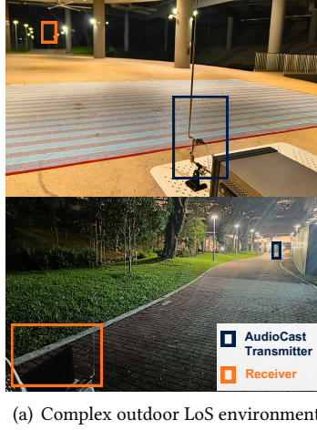
Fig. 18. Even in the presence of ambient FM-broadcasts and when AUDIOCAST signal propagates through complex environments—including buildings and vegetation—AUDIOCAST maintains high link quality. AUDIOCAST successfully transmits data over distances up to 110 meters, achieving a received strength of -109 dBm, a PRR of 0.89, and a BER of 0.1067. These metrics are sufficient to support a variety of outdoor applications, such as networking sensors in farms or cities.
