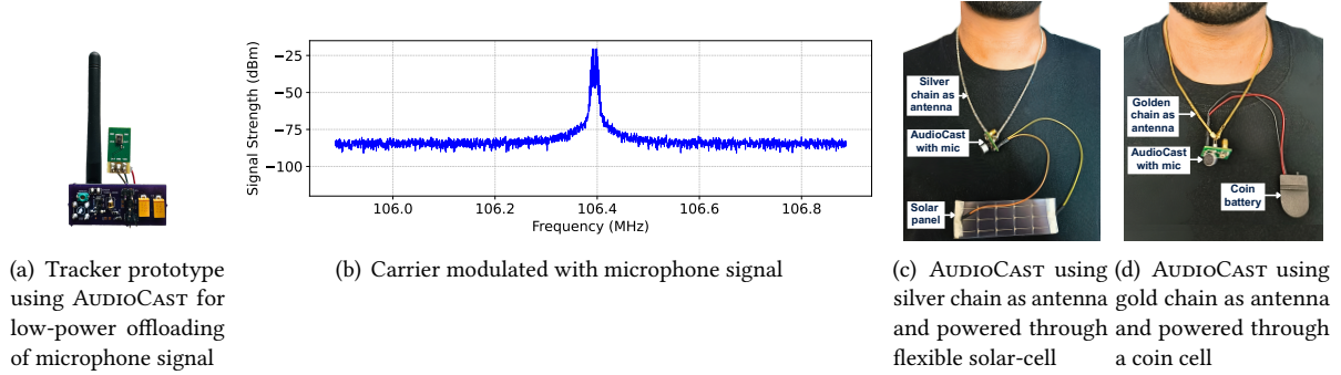
Fig. 22. AUDIOCAST enables the realization of a tracker for monitoring vocal interactions. A microphone is coupled with the AUDIOCAST transmitter, which directly modulates the carrier signal to produce a frequency-modulated signal. Commodity FM-radio receivers can then receive this signal. The FM-broadcast spectrum’s lower wavelength and favourable propagation properties allow the use of chains or wires as antennas, enabling efficient signal transmission.
